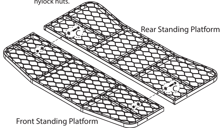
FIG. 1 STEP 1. Attach the front and rear standing platforms using (2) 1/4" x 1 3/4" hex bolts [C], (4) nylon washers and (2) 1/4" nylock nuts.
