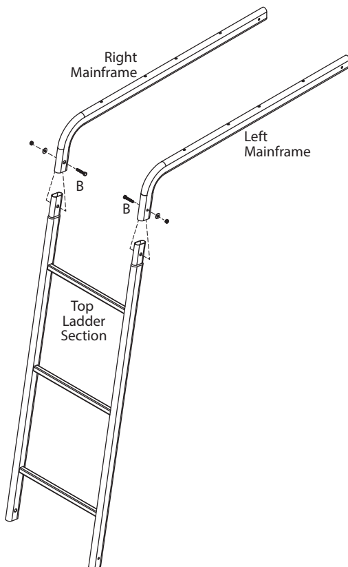
FIG. 2 STEP 2. Next, attach the left and right mainframes to a ladder section using (2) 1/4" x 1 1/2" hex bolts [B], (2) nylon washers and (2) 1/4" nylock nuts.
