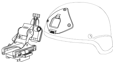
Titanium Advanced Tactical Helmet Mount Assembly
