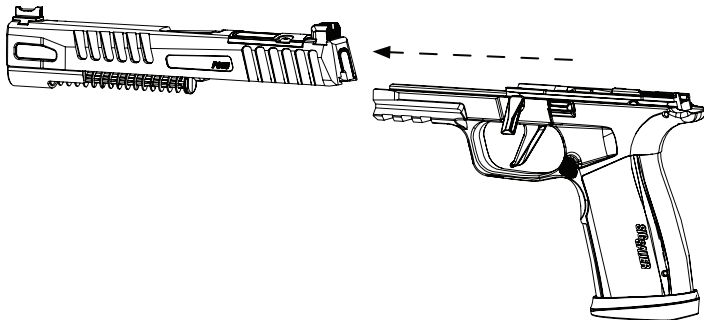
Figure 1. Remove Slide.
