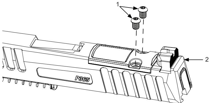
Figure 2. Remove Sight Plate Screw.
